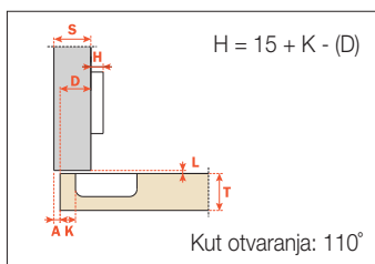
Push-open adapter
